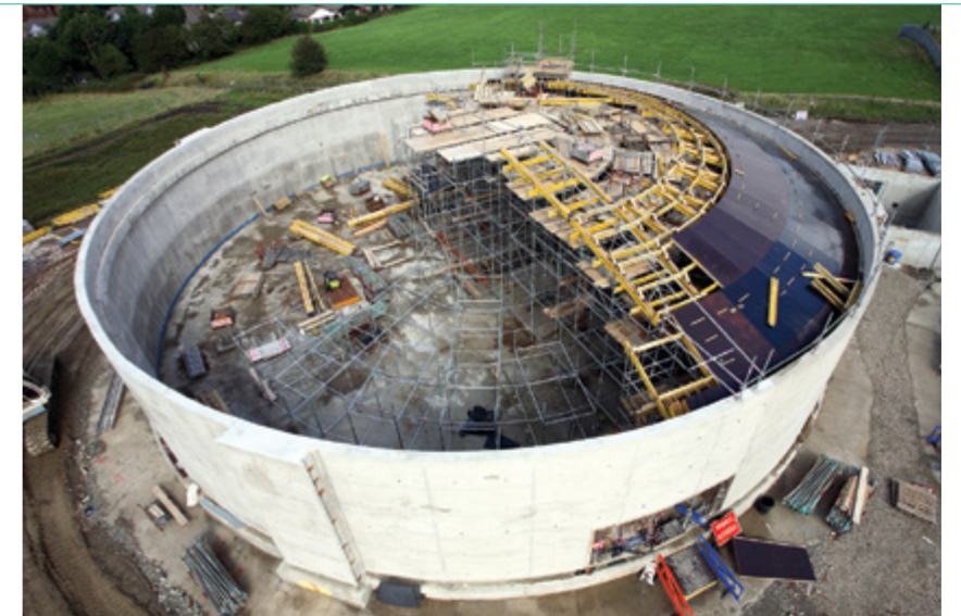
'TOP OF THE COW' – POST TENSION INSTALLATION AS PART OF TANK CONSTRUCTION
